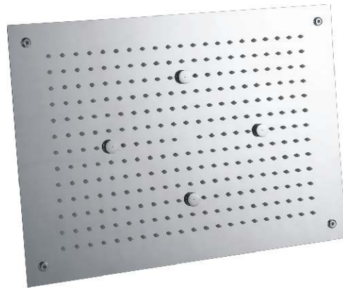
Code : 8276 MRP : ₹ 19,900/- Two-Function Ceiling Shower 2 Functions ( Rain + Mist) Material : SS 304 (Mirror Finish) Size : 480 X 330mm (19"x13")
